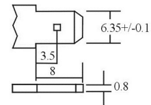
Optional Terminal B1(copper) Bolt Type:M5
