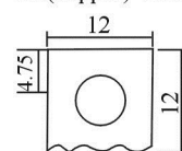
Optional Terminal B1(copper) Bolt Type:M5
