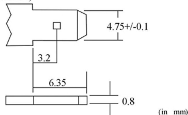
Standard Terminal F3 (Fasten Tab No.187A)
