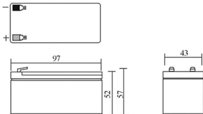
Dimensions (mm)
