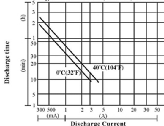
Discharge Characteristics (0°C/32°F, 40°C/104°F)
