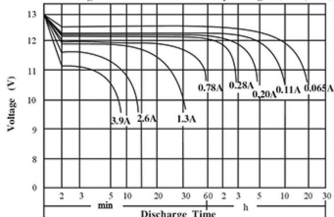
Discharge Characteristics after fully charged (25°C,77°F)
